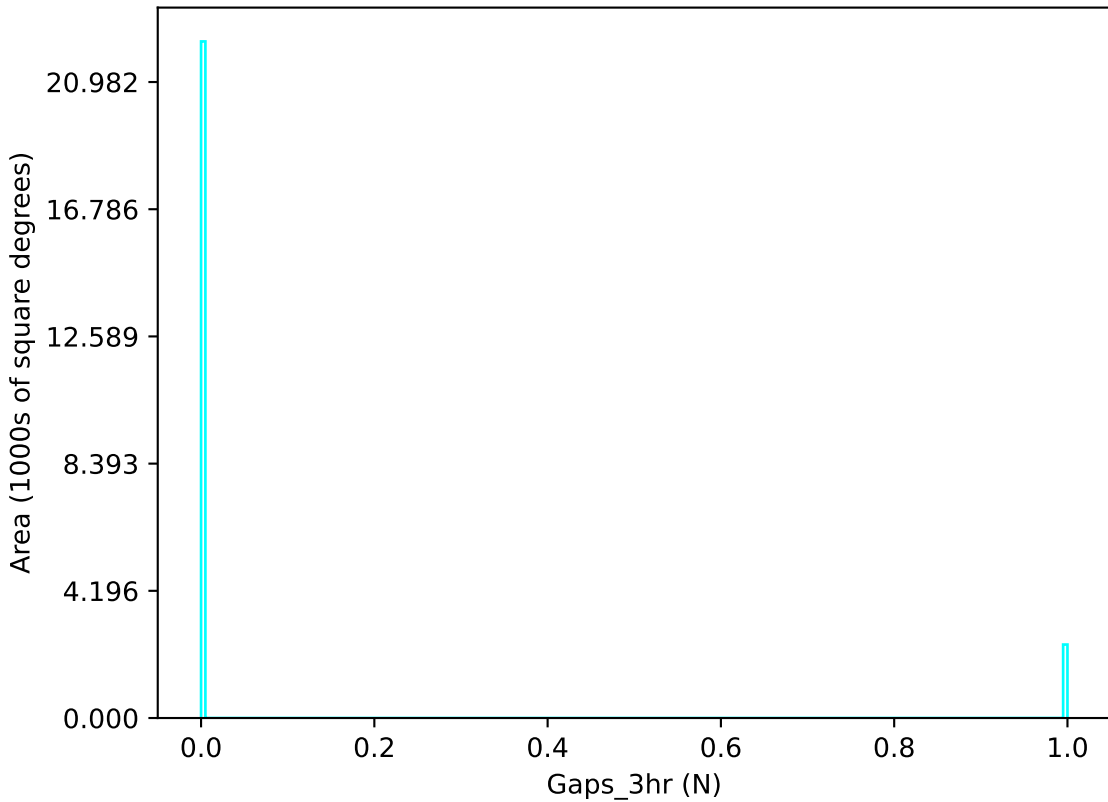
too_100_1v3.4_10yrs u band: Gaps_3hr
