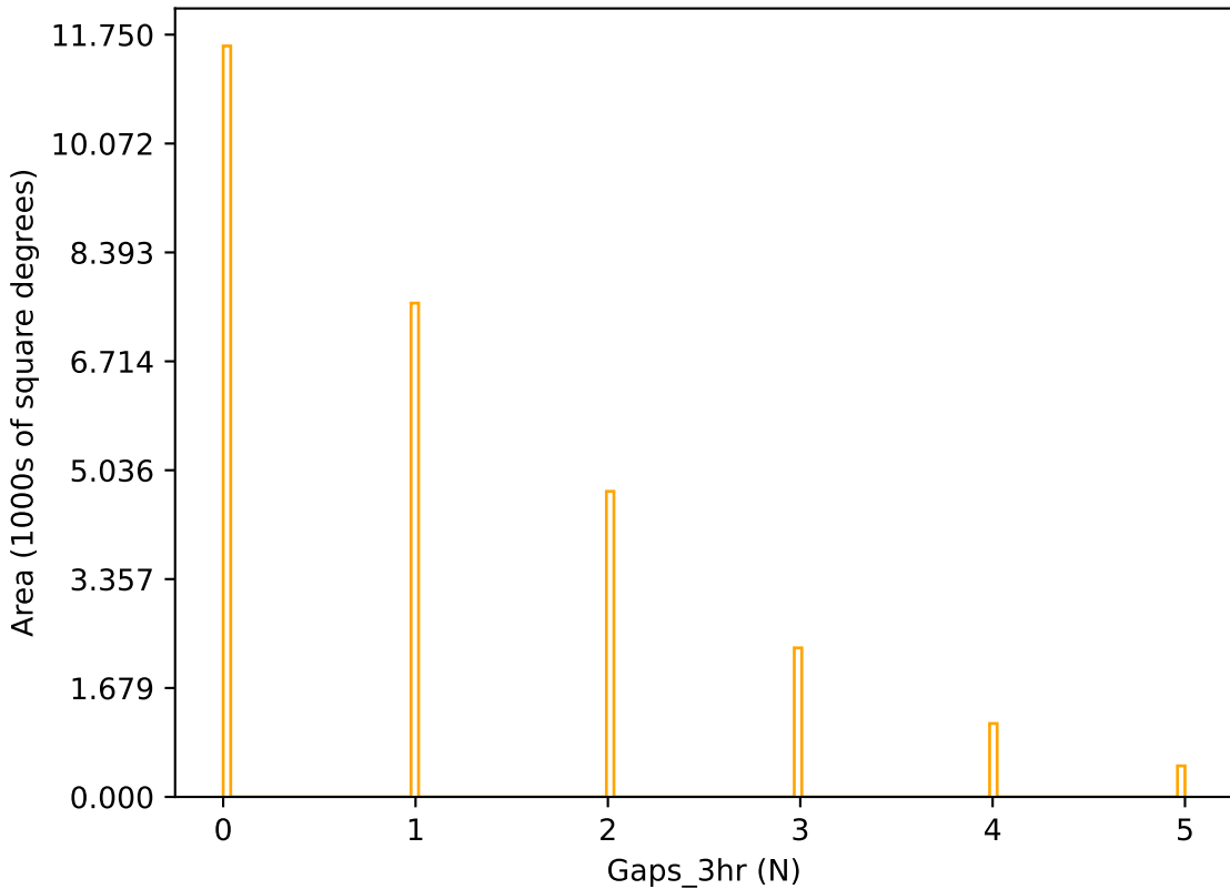
too_100_1v3.4_10yrs r band: Gaps_3hr
