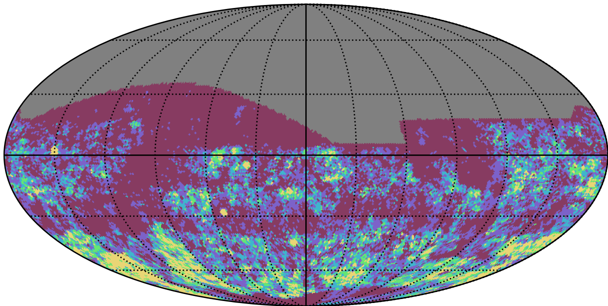
too_100_1v3.4_10yrs i band: Gaps_3hr
