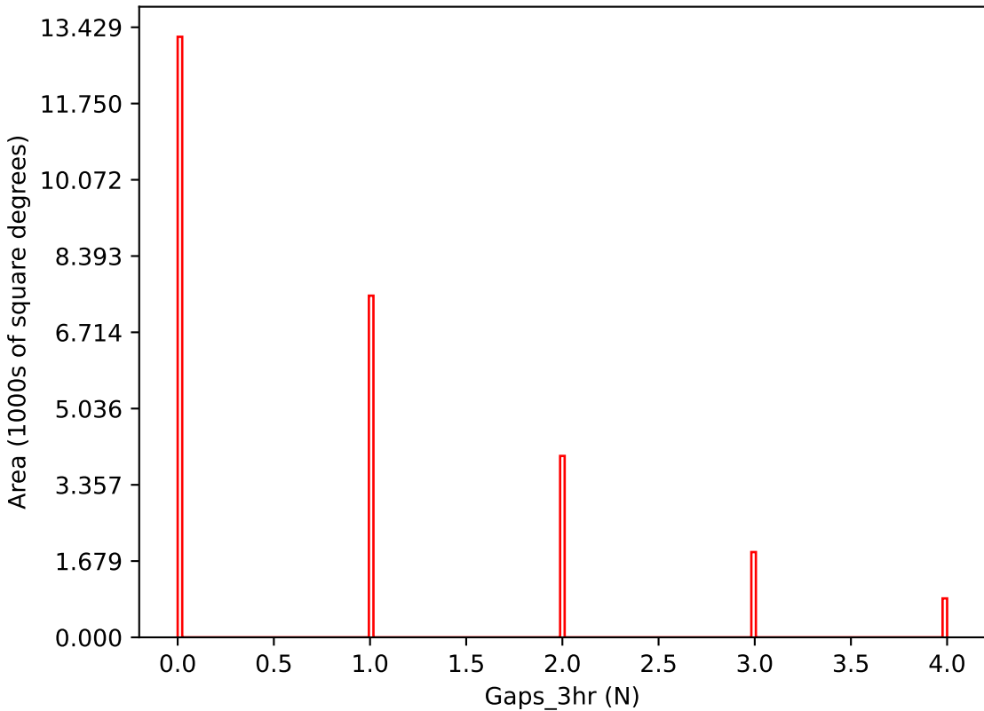
too_100_1v3.4_10yrs i band: Gaps_3hr
