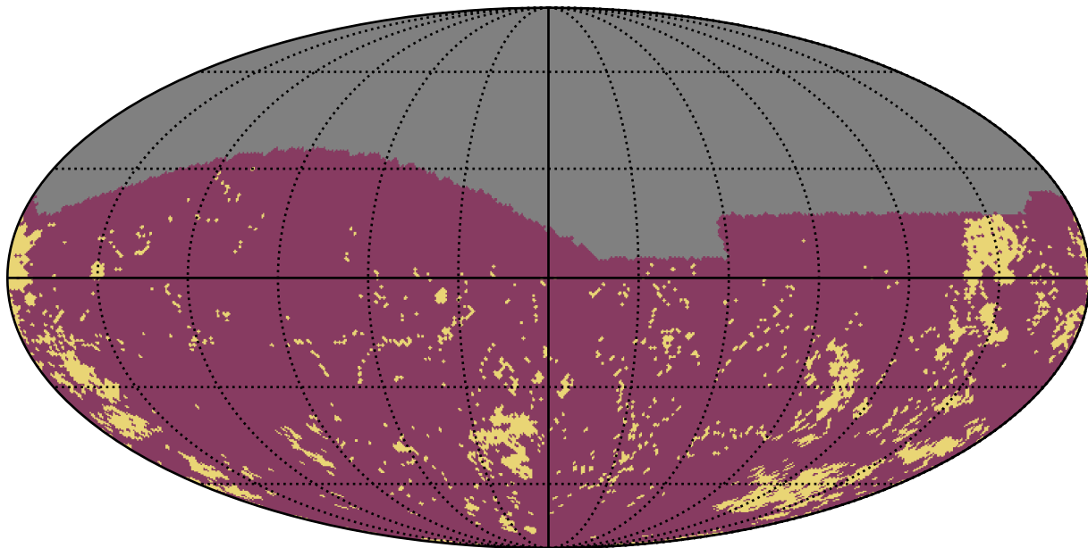
too_100_1v3.4_10yrs g band: Gaps_3hr
