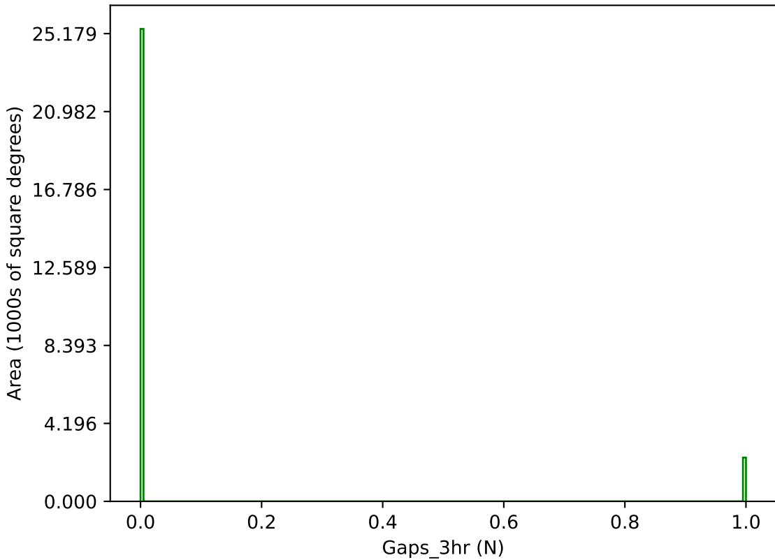
too_100_1v3.4_10yrs g band: Gaps_3hr
