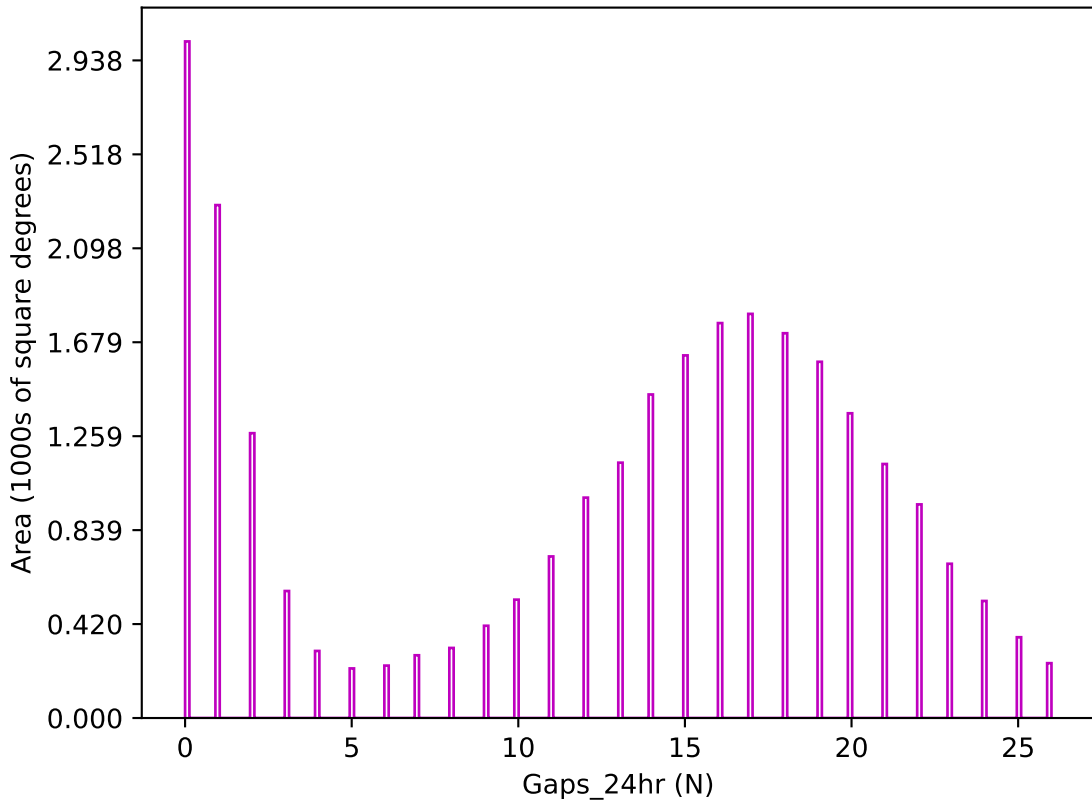
too_100_1v3.4_10yrs z band: Gaps_24hr
