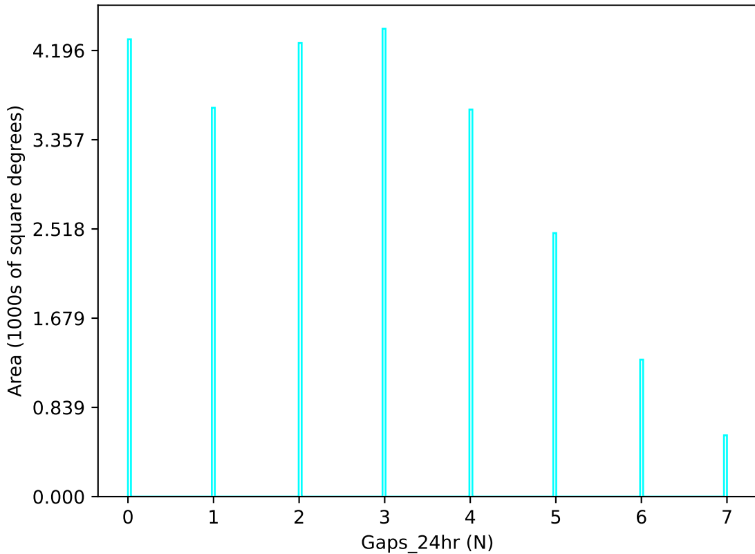
too_100_1v3.4_10yrs u band: Gaps_24hr
