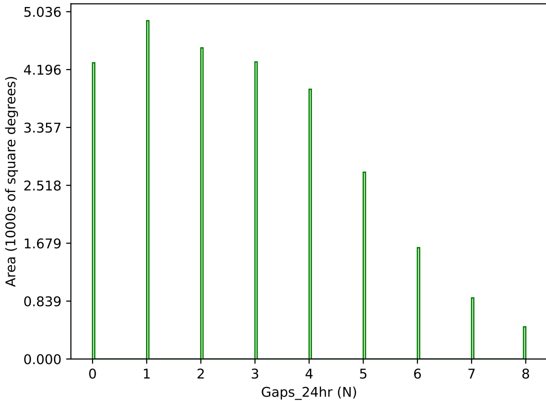
too_100_1v3.4_10yrs g band: Gaps_24hr
