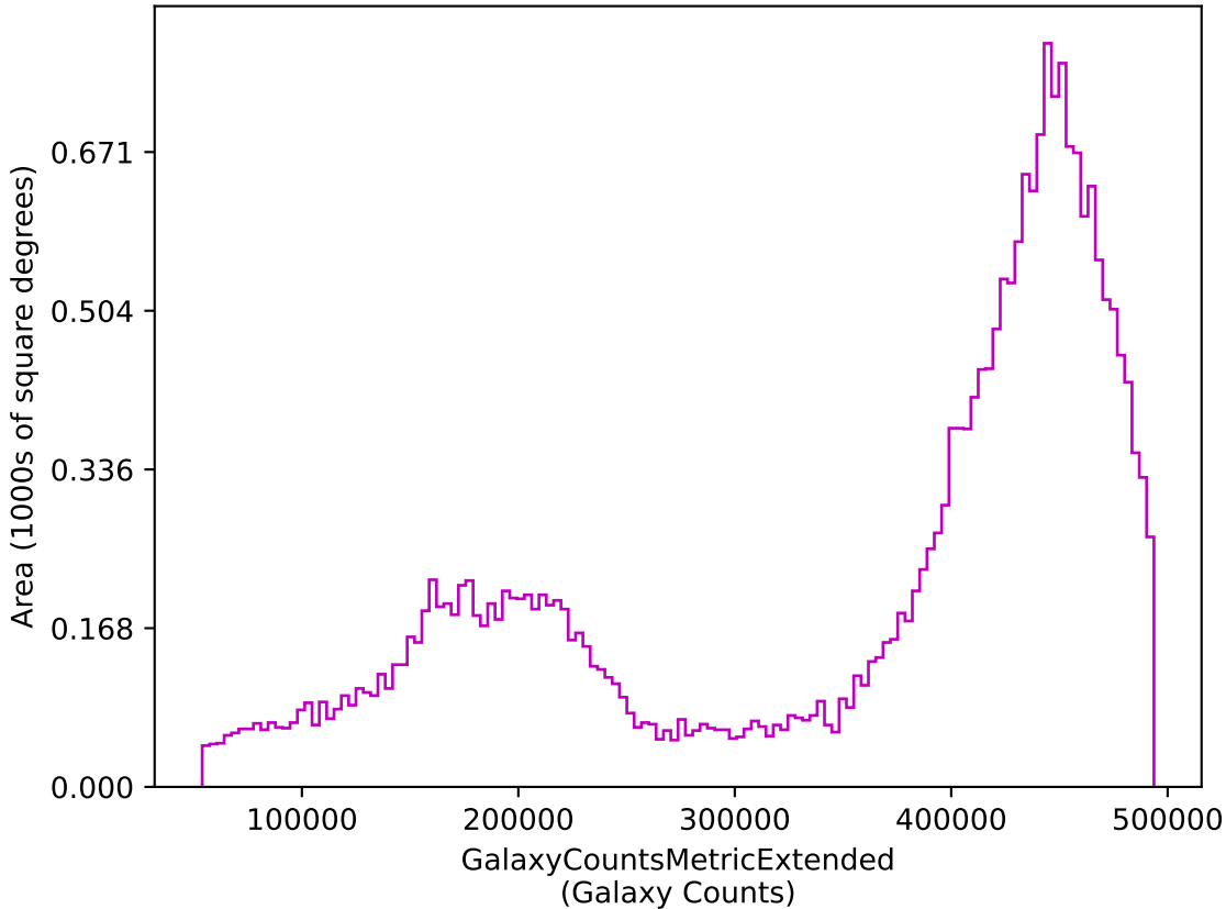
too_100_1v3.4_10yrs z: GalaxyCountsMetricExtended
