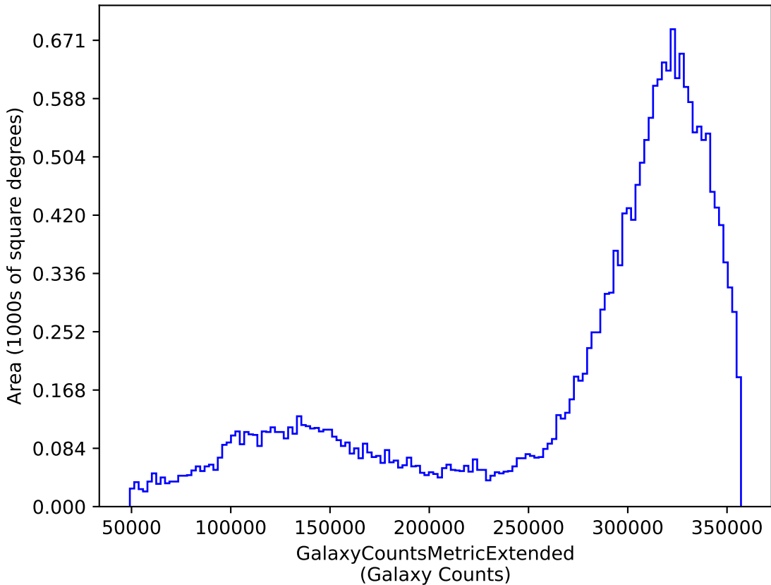
too_100_1v3.4_10yrs y: GalaxyCountsMetricExtended
