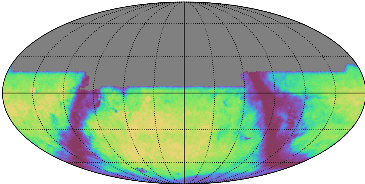
too_100_1v3.4_10yrs u: GalaxyCountsMetricExtended
