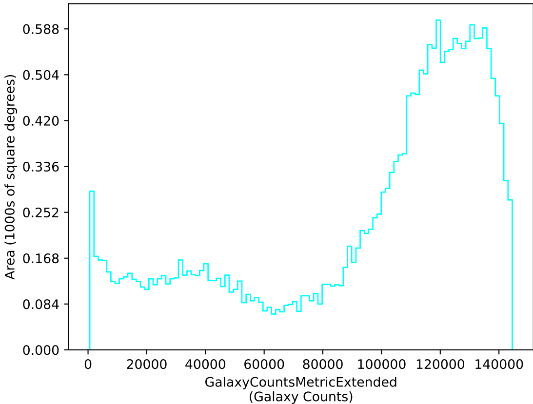
too_100_1v3.4_10yrs u: GalaxyCountsMetricExtended
