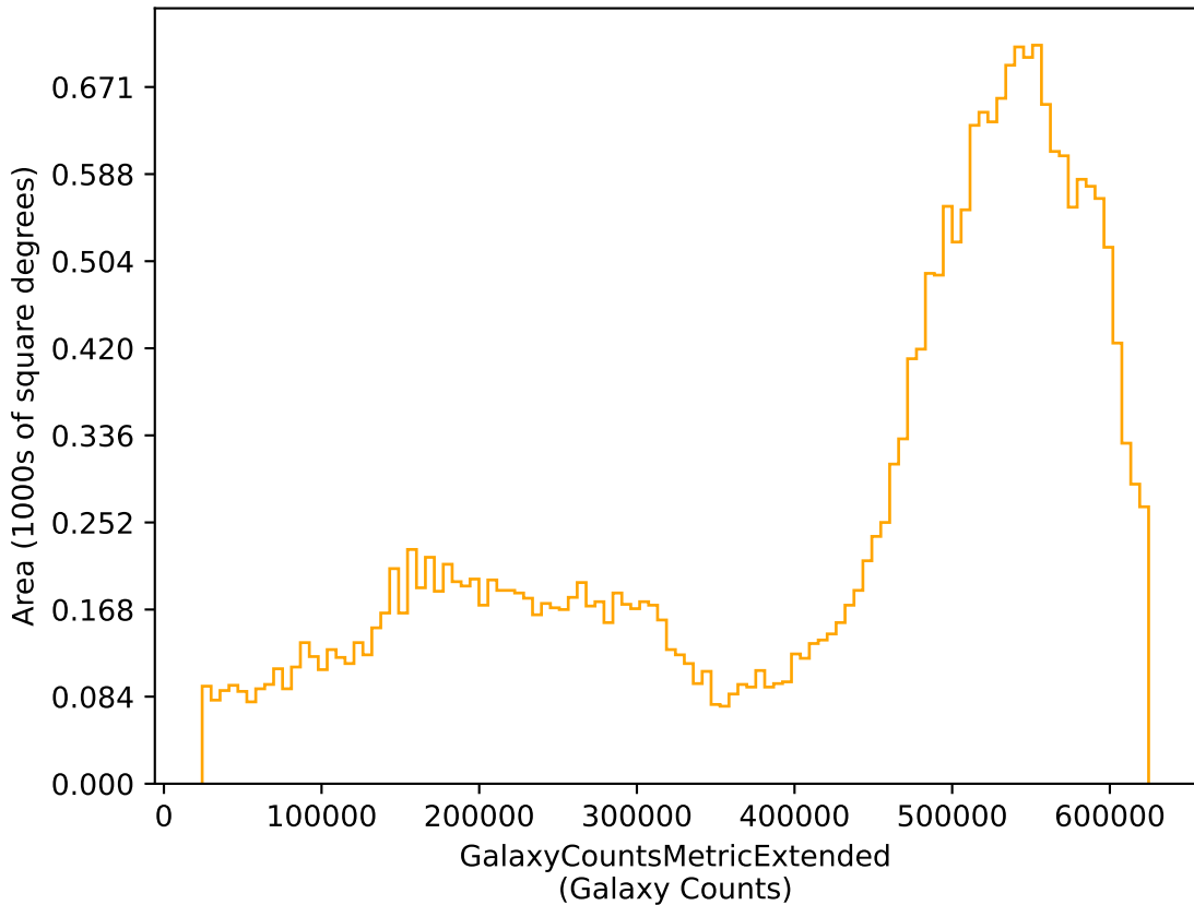
too_100_1v3.4_10yrs r: GalaxyCountsMetricExtended
