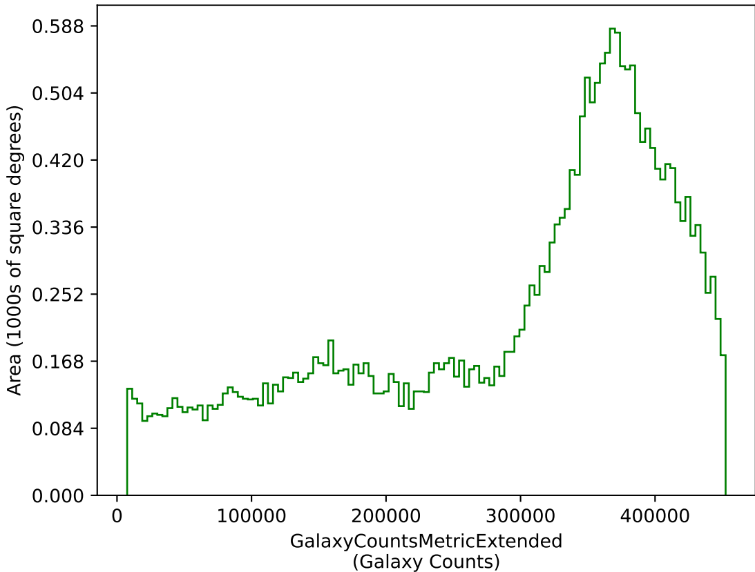
too_100_1v3.4_10yrs g: GalaxyCountsMetricExtended
