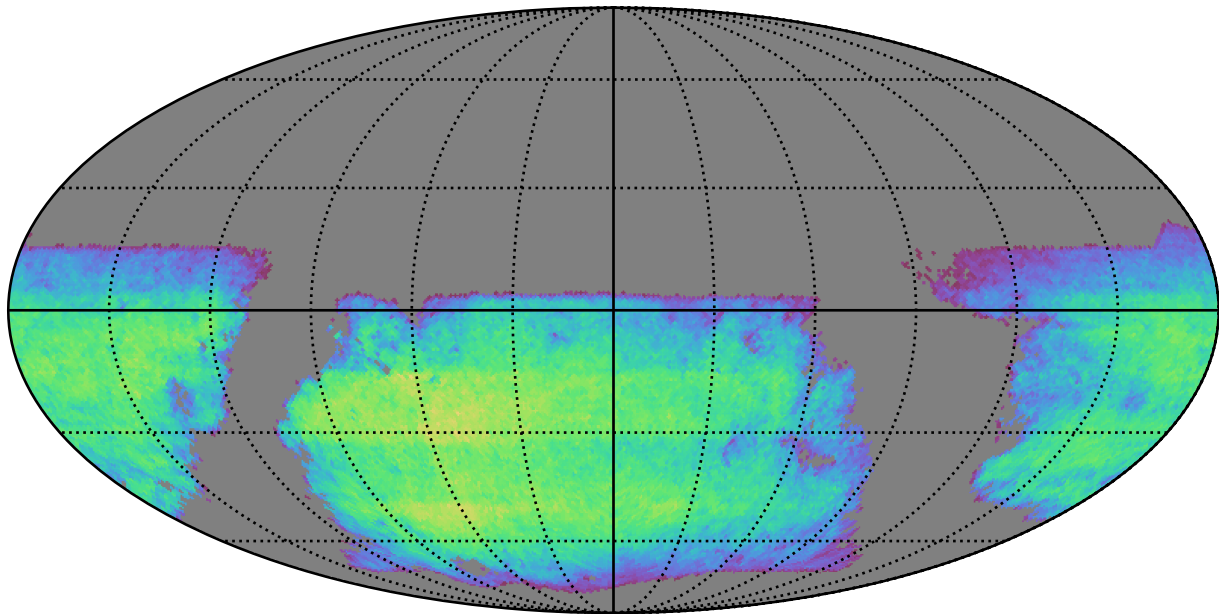
too_100_1v3.4_10yrs i band non-DD year 9: ExgalM5WithCuts
