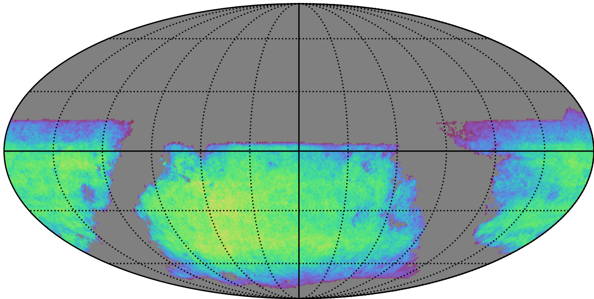
too_100_1v3.4_10yrs i band non-DD year 8: ExgalM5WithCuts
