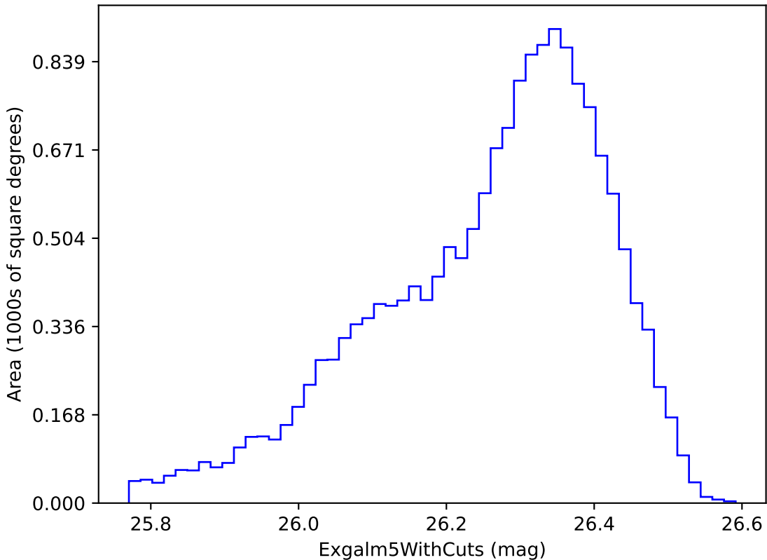
too_100_1v3.4_10yrs i band non-DD year 8: ExgalM5WithCuts
