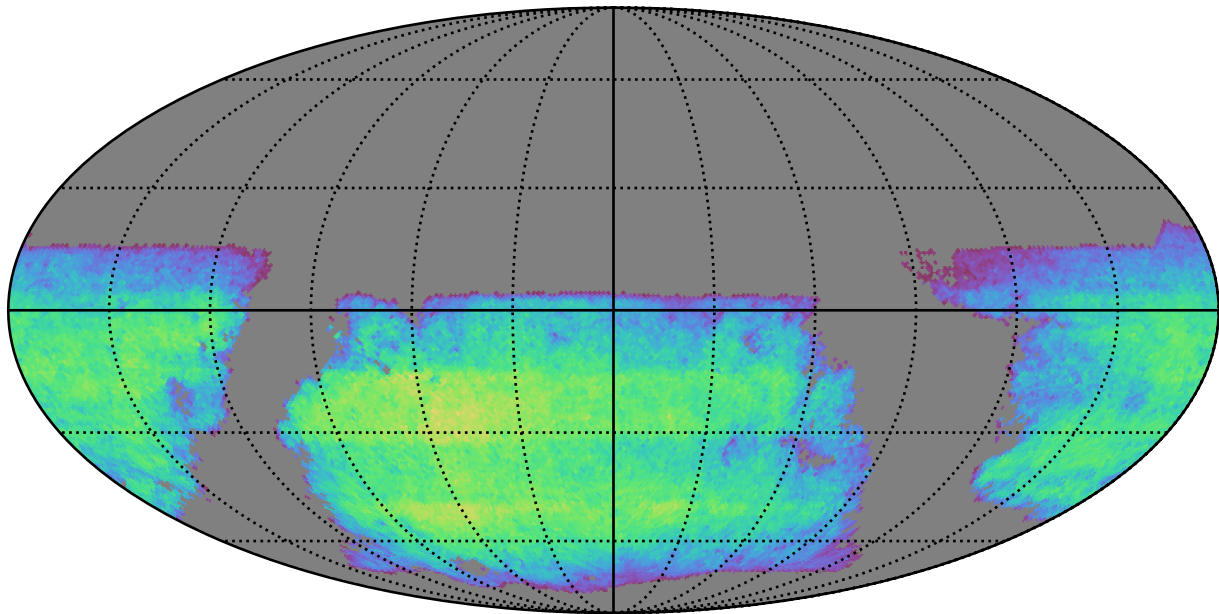
too_100_1v3.4_10yrs i band non-DD year 7: ExgalM5WithCuts
