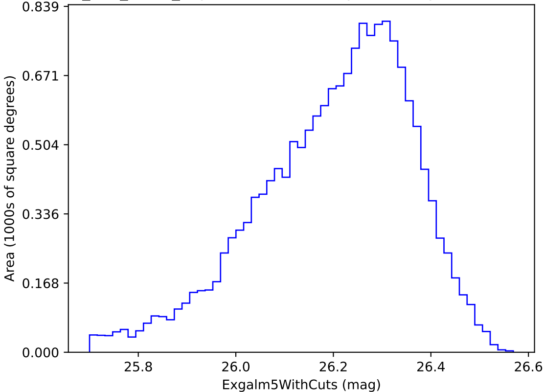
too_100_1v3.4_10yrs i band non-DD year 7: ExgalM5WithCuts
