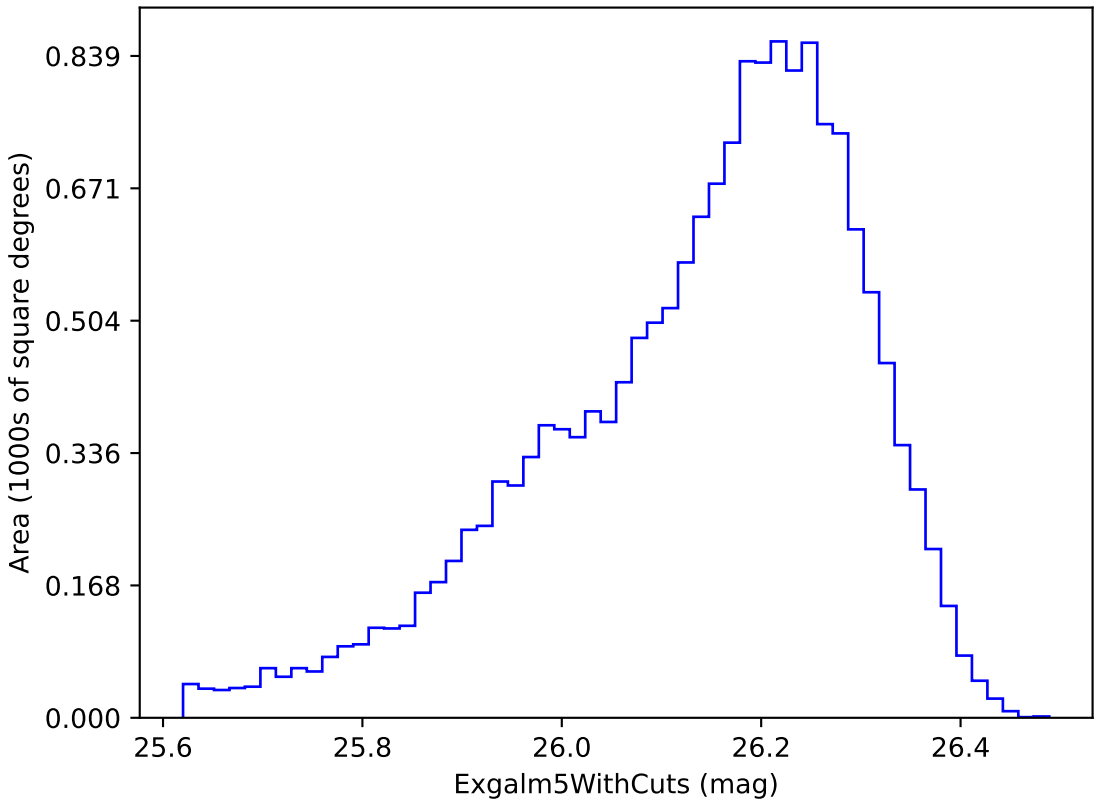
too_100_1v3.4_10yrs i band non-DD year 6: ExgalM5WithCuts
