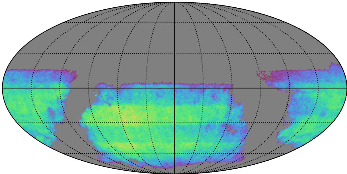
too_100_1v3.4_10yrs i band non-DD year 5: ExgalM5WithCuts
