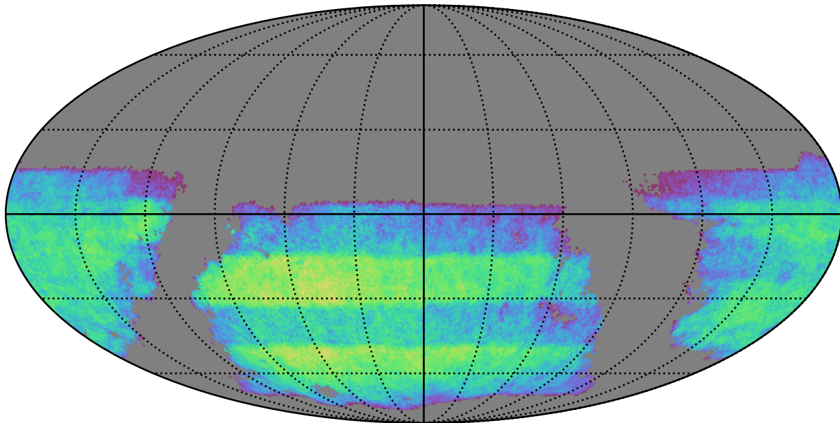
too_100_1v3.4_10yrs i band non-DD year 3: ExgalM5WithCuts
