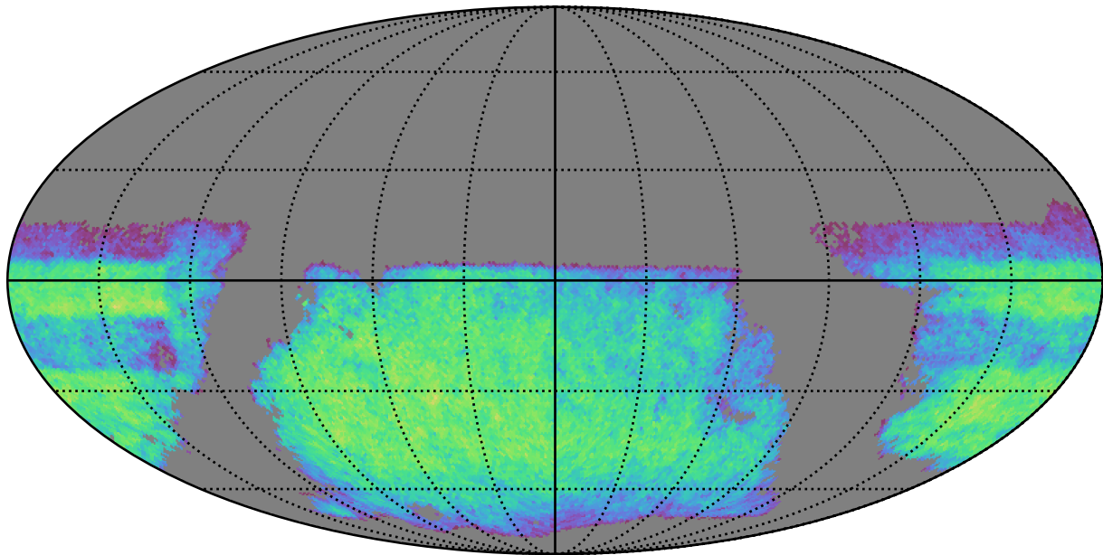
too_100_1v3.4_10yrs i band non-DD year 2: ExgalM5WithCuts
