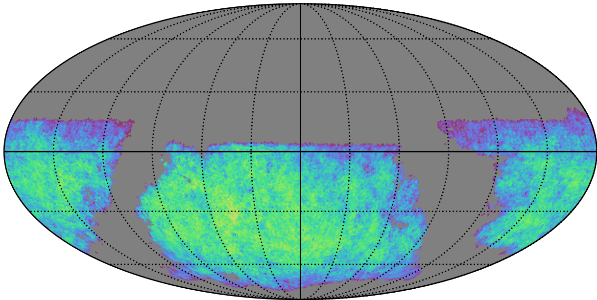
too_100_1v3.4_10yrs i band non-DD year 1: ExgalM5WithCuts
