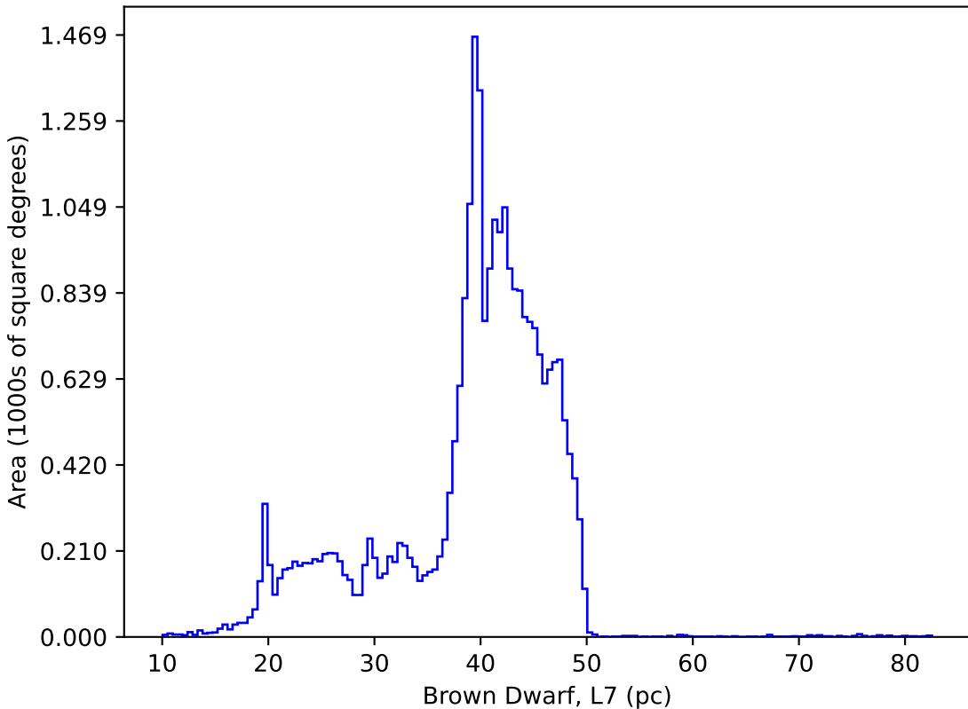
too_100_1v3.4_10yrs : Brown Dwarf, L7
