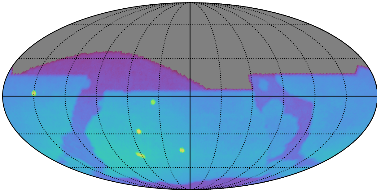
too_100_1v3.4_10yrs : Brown Dwarf, L4
