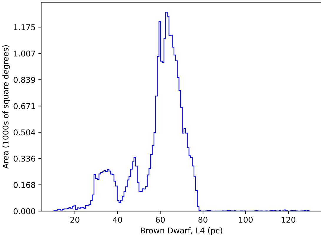
too_100_1v3.4_10yrs : Brown Dwarf, L4
