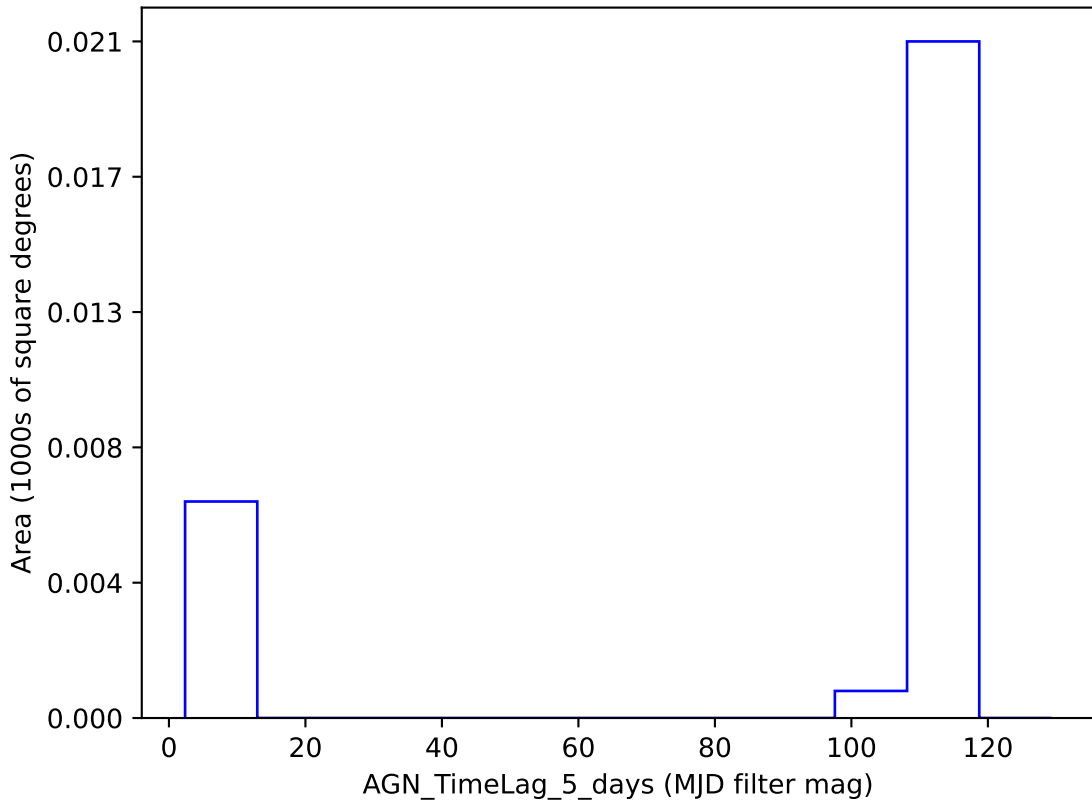
too_100_1v3.4_10yrs y band: AGN_TimeLag_5_days
