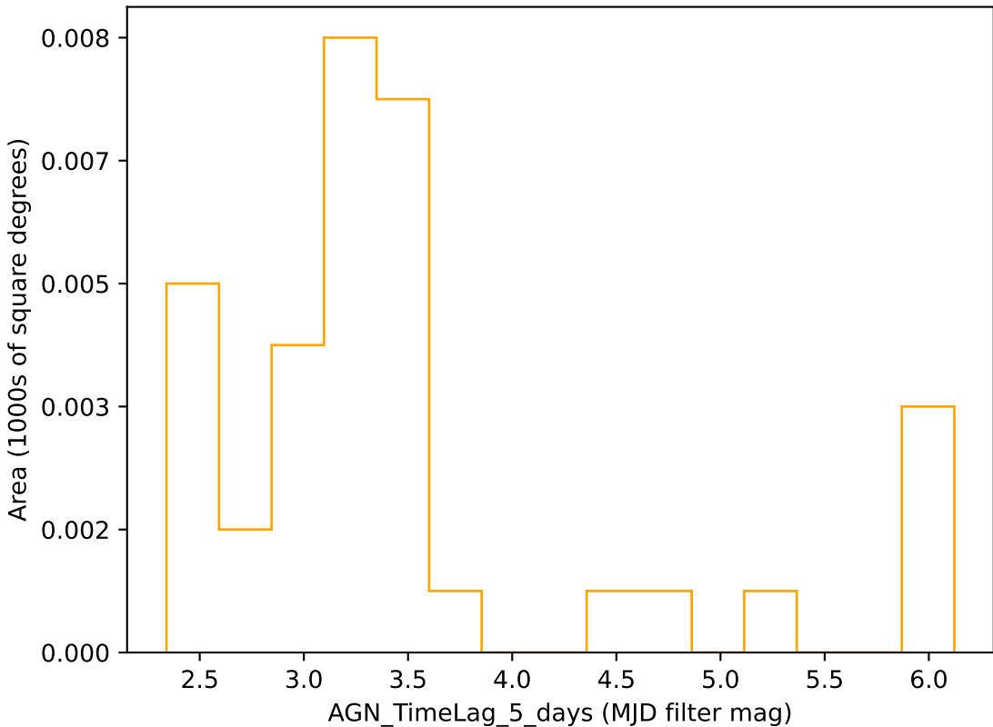
too_100_1v3.4_10yrs r band: AGN_TimeLag_5_days
