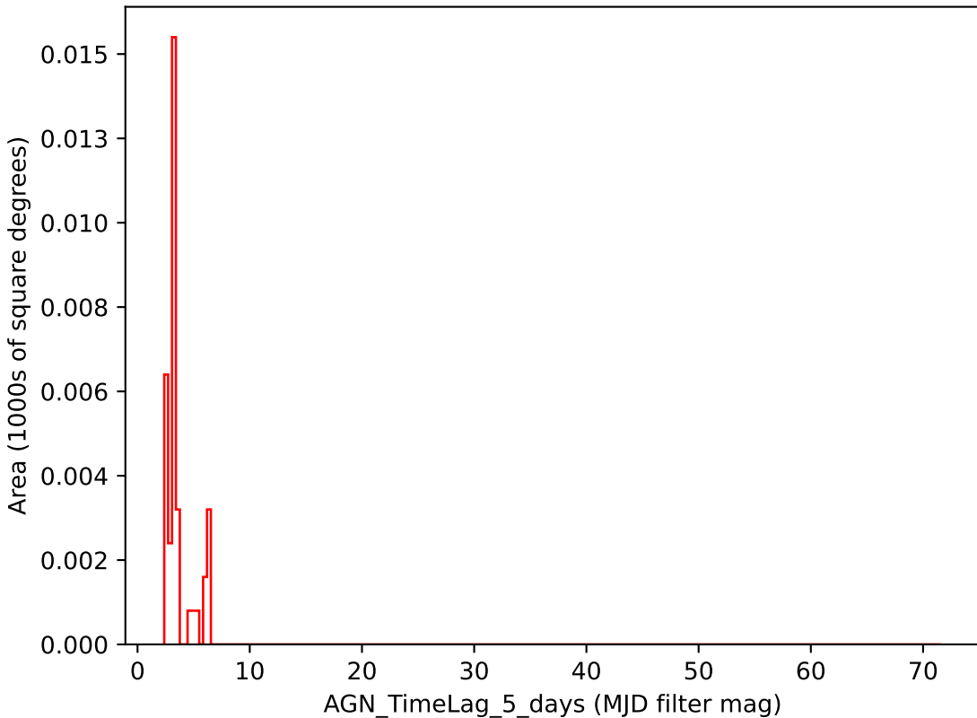
too_100_1v3.4_10yrs i band: AGN_TimeLag_5_days
