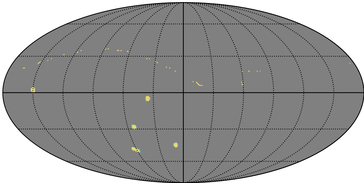
too_100_1v3.4_10yrs all bands: AGN_TimeLag_5_days
