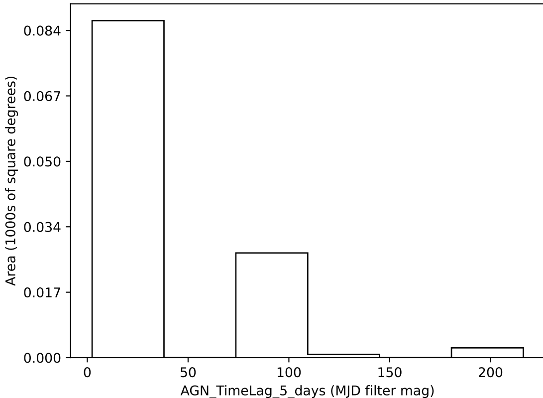
too_100_1v3.4_10yrs all bands: AGN_TimeLag_5_days
