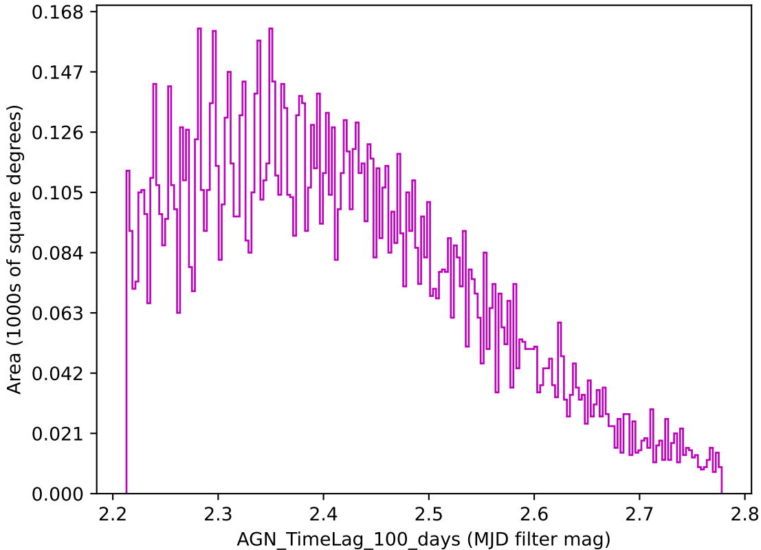
too_100_1v3.4_10yrs z band: AGN_TimeLag_100_days
