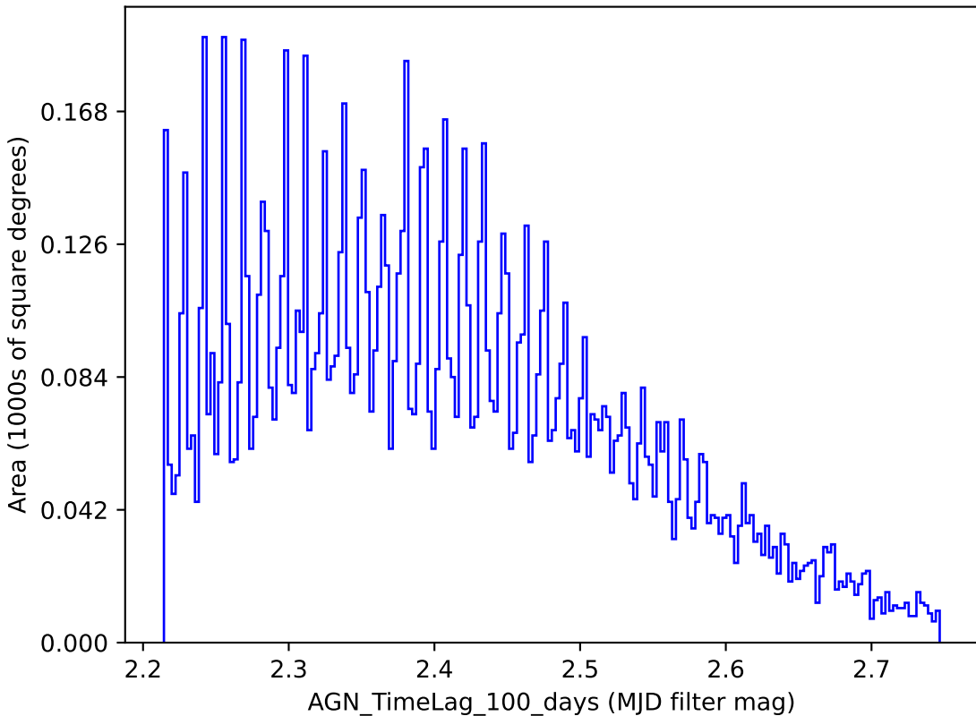
too_100_1v3.4_10yrs y band: AGN_TimeLag_100_days
