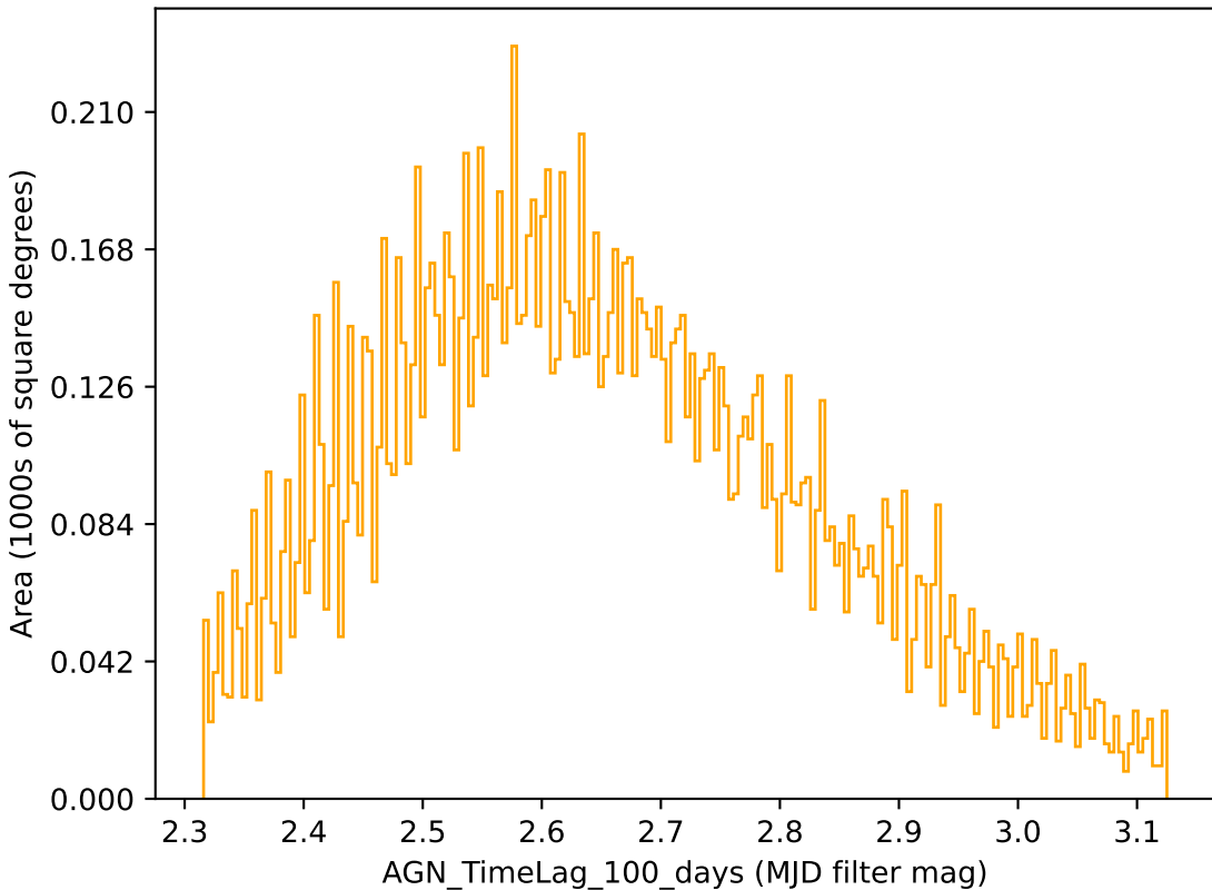
too_100_1v3.4_10yrs r band: AGN_TimeLag_100_days
