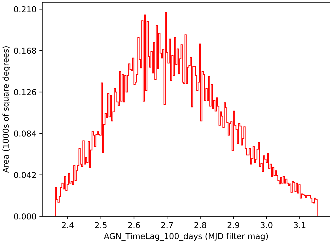
too_100_1v3.4_10yrs i band: AGN_TimeLag_100_days
