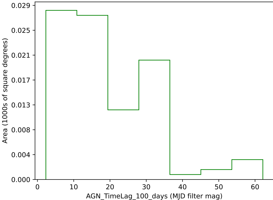
too_100_1v3.4_10yrs g band: AGN_TimeLag_100_days
