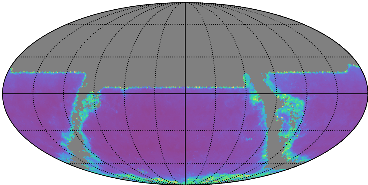
too_100_1v3.4_10yrs y band: AGN SF_uncert
