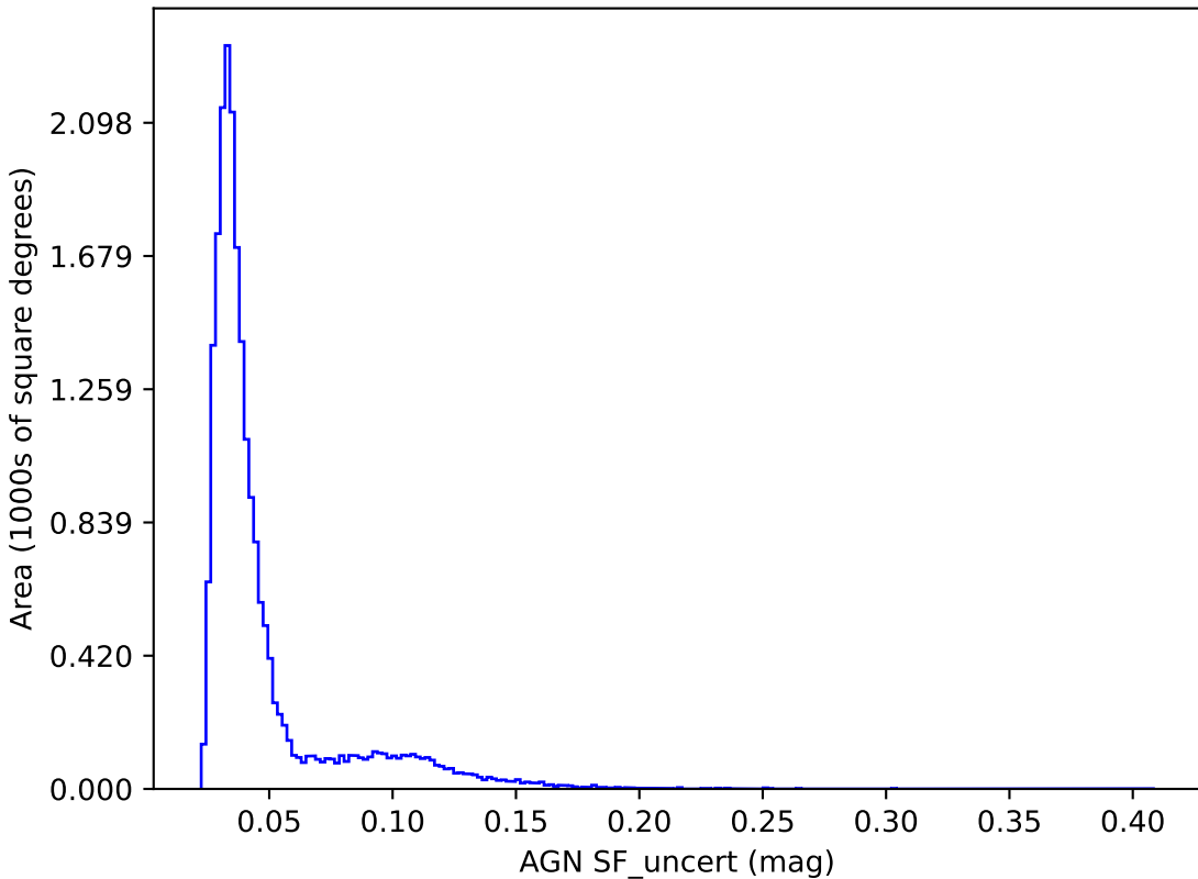
too_100_1v3.4_10yrs y band: AGN SF_uncert
