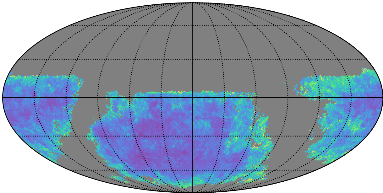
too_100_1v3.4_10yrs u band: AGN SF_uncert
