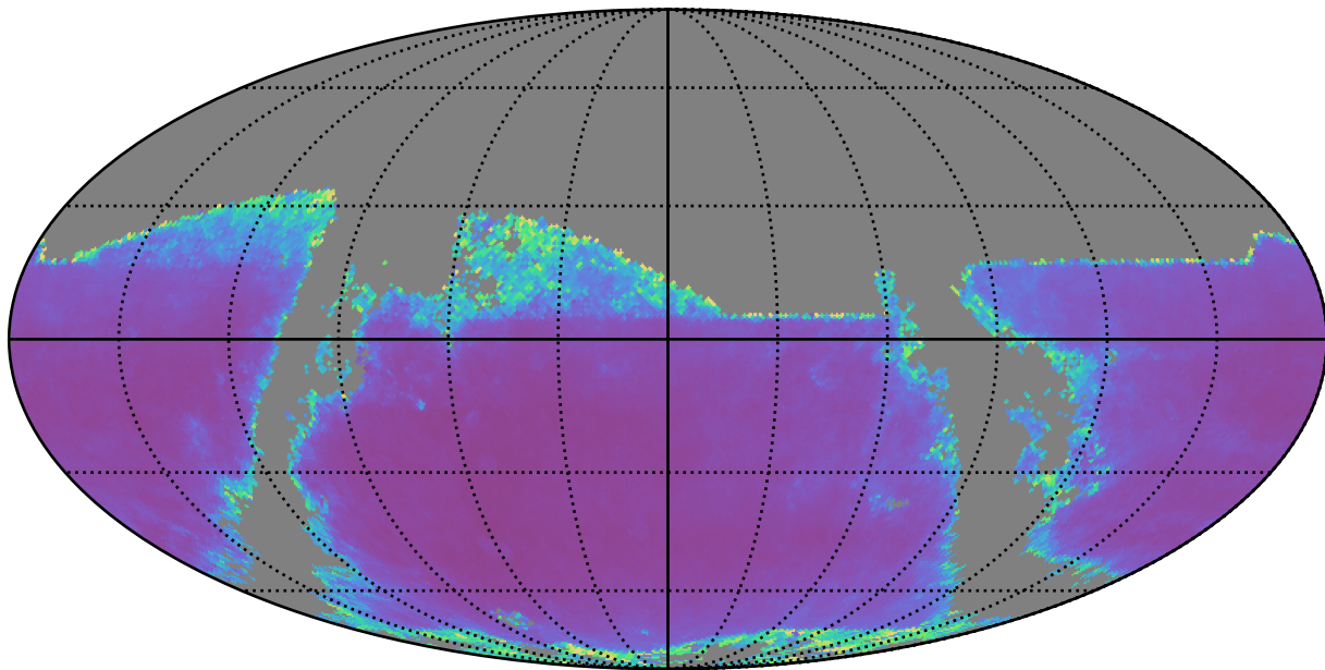
too_100_1v3.4_10yrs r band: AGN SF_uncert
