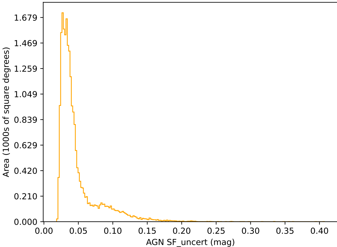
too_100_1v3.4_10yrs r band: AGN SF_uncert
