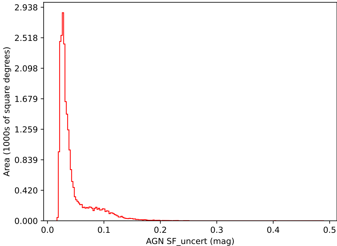
too_100_1v3.4_10yrs i band: AGN SF_uncert
