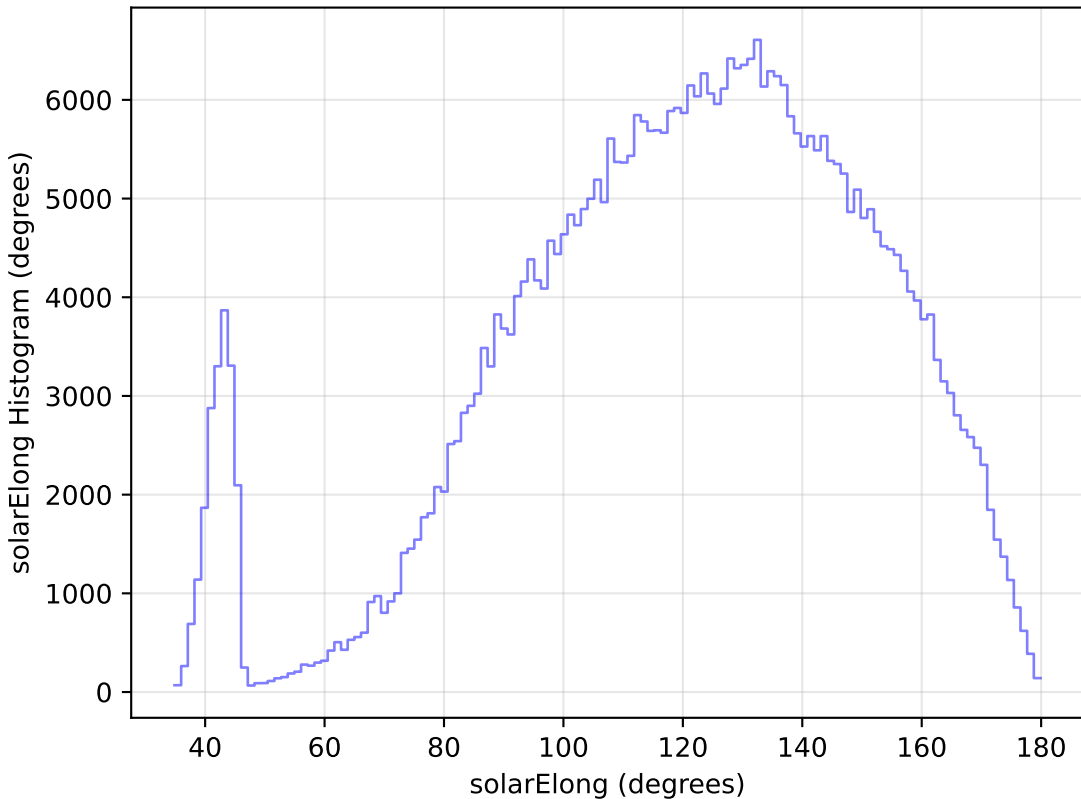
too_100_1v3.4_10yrs WFD z band: solarElong Histogram
