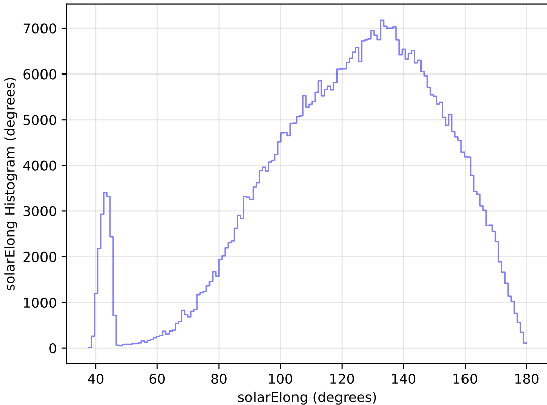
too_100_1v3.4_10yrs WFD r band: solarElong Histogram
