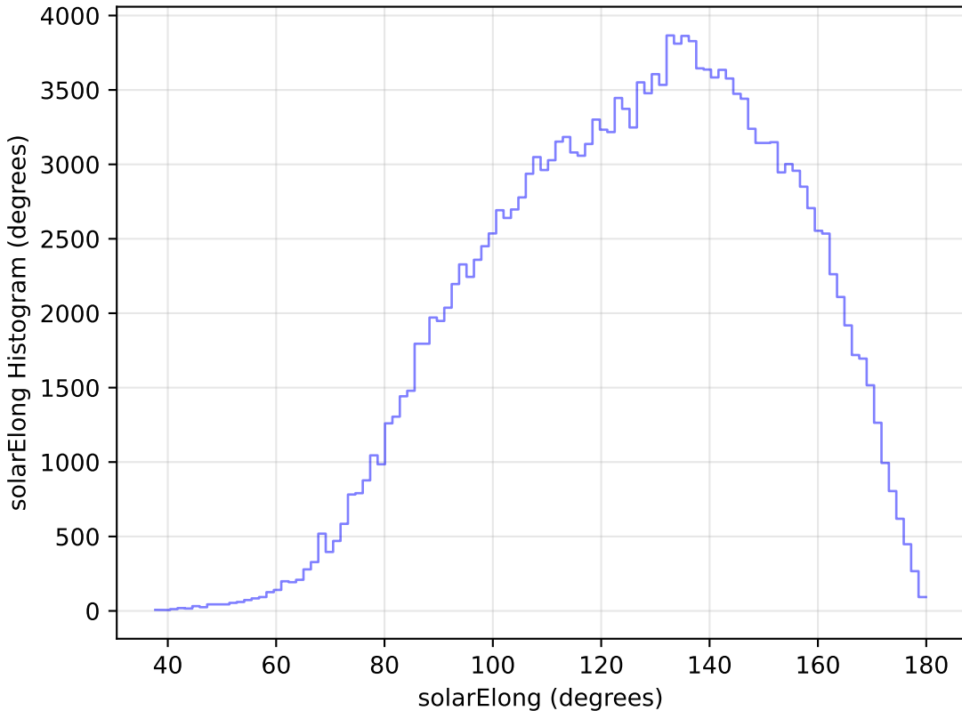
too_100_1v3.4_10yrs WFD g band: solarElong Histogram
