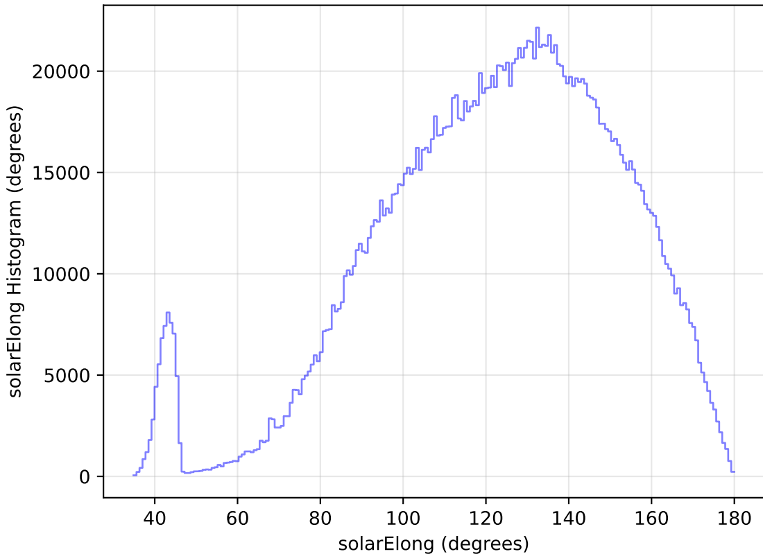
too_100_1v3.4_10yrs WFD all bands: solarElong Histogram
