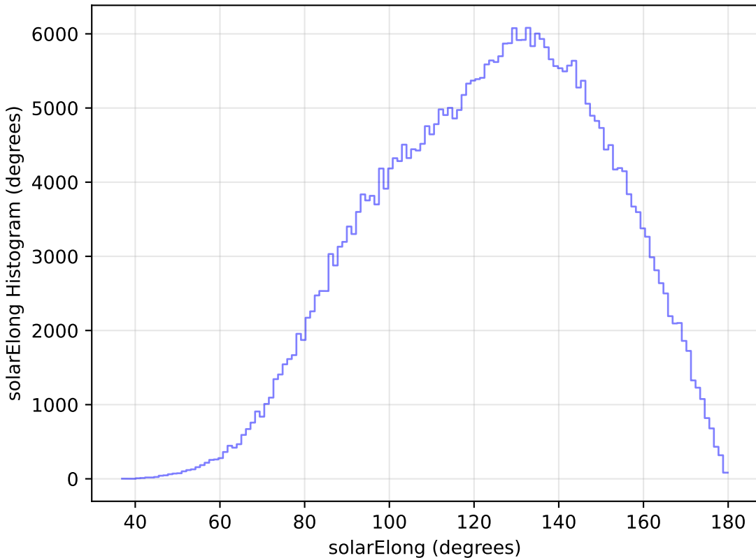
too_100_1v3.4_10yrs All sky y band: solarElong Histogram
