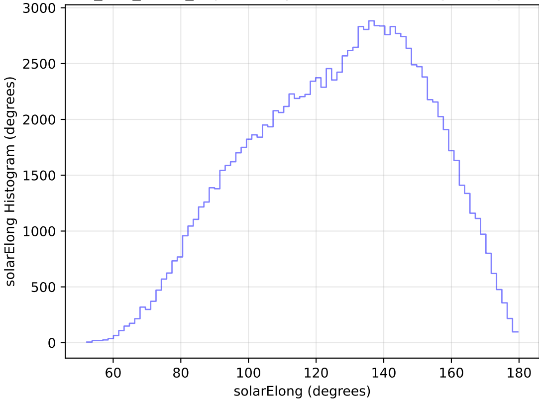
too_100_1v3.4_10yrs All sky u band: solarElong Histogram
